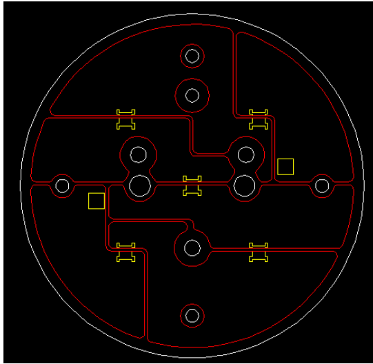
MCPCB Layout
