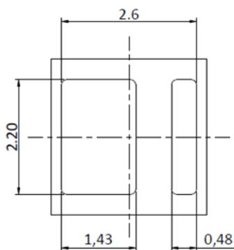
Bot. view
